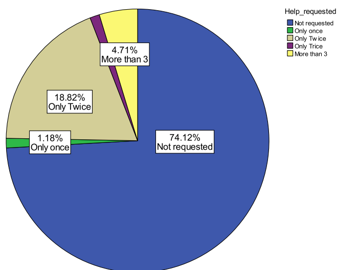
Figure 7. 5 Help Requested
