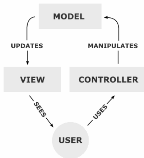
Figure 4. 5 MVC Framework
