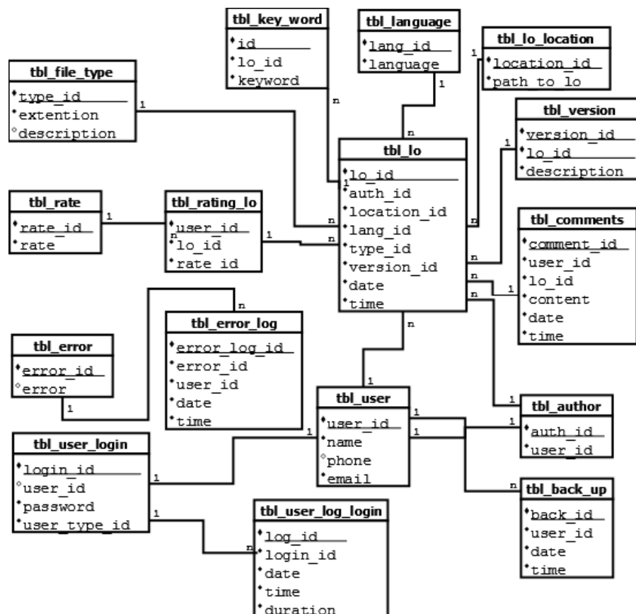
Figure 4. 7 Database diagram for HLOR
