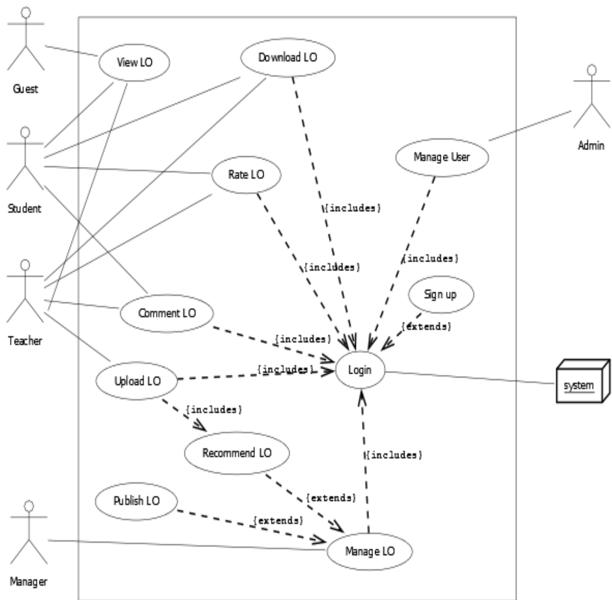
Figure 4. 1 High Level Use Case Diagram fro HLOR
