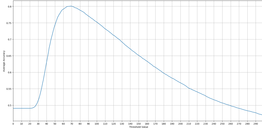
Figure 5.1: Average Accuracy Values for Different Threshold Values (Keypoint Count)
