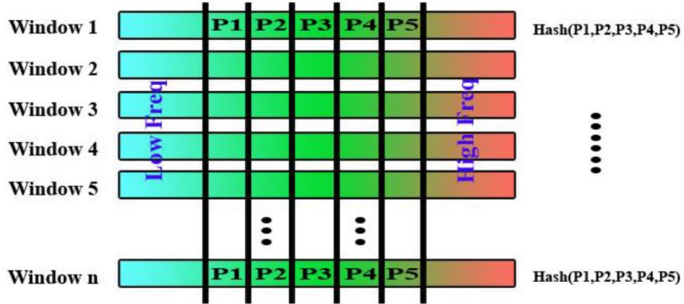
Figure 1.3: Extracting peaks and generating a hash value[1]
