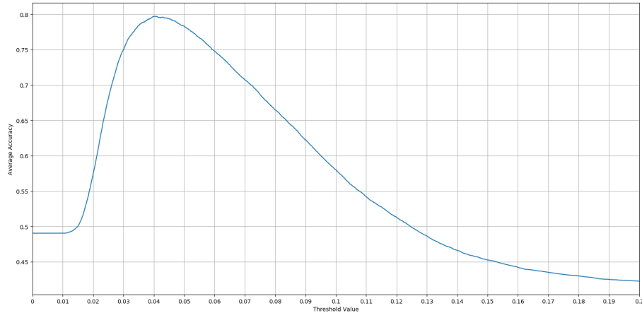
Figure 1.8: Average Accuracy Values for Different Threshold Values
