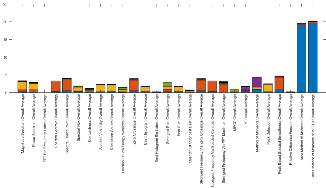
Figure 3.4: PCA coefficients weighted by eigen values (Normalized by Rescaling)
