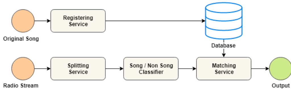
Figure 1.2: Architecture of the existing system
