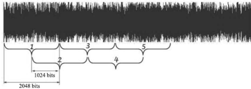
Figure 3.6: Key parameters on STFT. 2048 bits long window with 1024 bits long overlapping area.
