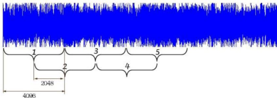
Figure 1.1: Key controlling parameters of STFT[1]
