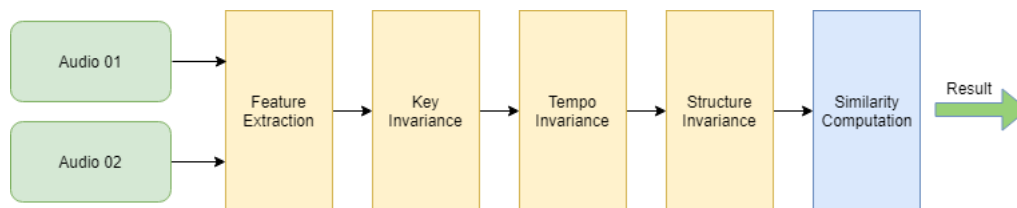
Figure 2.1: General Pipeline for Cover Song Identification
